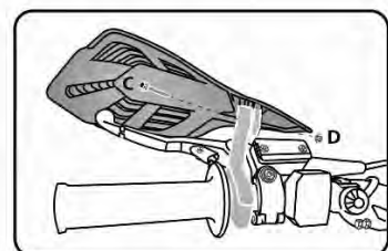
3- Insert and tighten the screw C and the nut (D) to attach the shields to the mount. Check the bolts (B) on the mount to ensure they are also tight.
