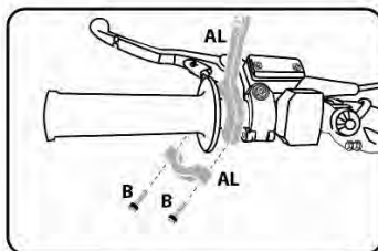
1- Attach the Left side mount (AL) to the handlebar using the screws (B).
