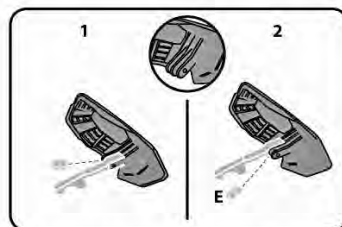
2- Depending on your mounting location on the bars, attach the shields to the mounts utilizing the internal or external mounting points.
