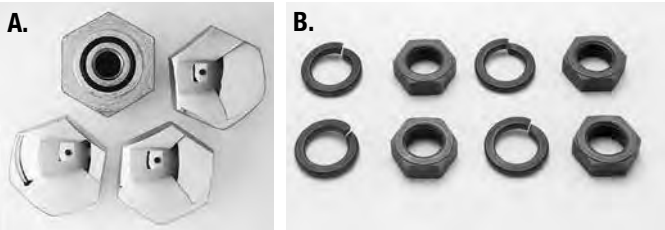
A. Knuckle Nut Set Duplicate of original Harley part except for the addition of a positive "O" ring seal to prevent oil leakage. Contains 4 nuts and 4 seals. Fits all Knucklehead engines 1936-1947. Stock No. 7110-8
