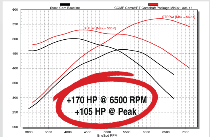
Stage 3 MK201-306-17 HRT™ Cam Package tested on a stock 6.4L engine with long tube headers, valve train upgrades and FAST® 87mm Big Mouth LT Throttle Body™.
