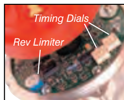
Timing curve and the rev limit adjustments are made with the rotary dials beneath the rotor. See page 99 for timing curve samples.
