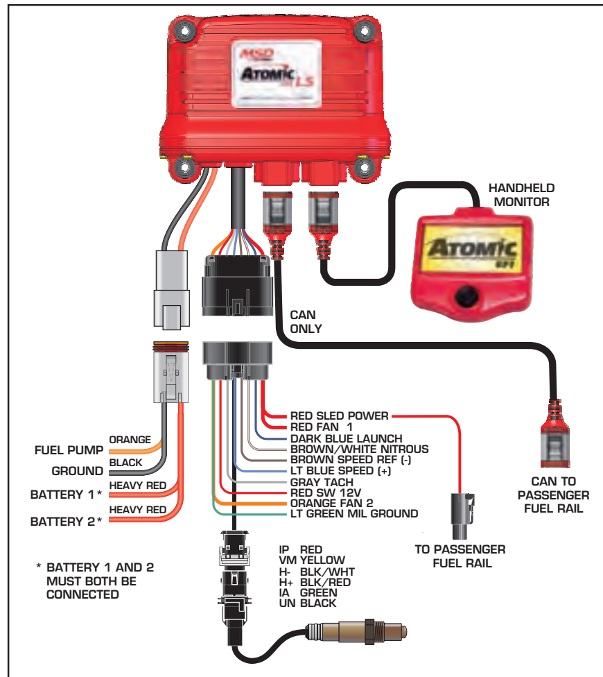
This diagram shows the Power Module Wiring.
