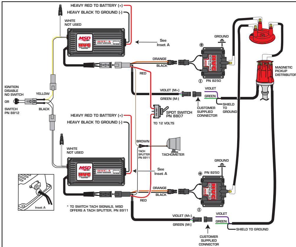
This diagram shows a professional racing system with dual HVC-L ignitions, coils and distributor.
