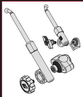
QuickSet™ for Street Shield™
