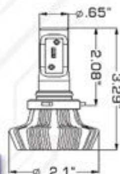
H10 LED HEADLIGHT BULBS
