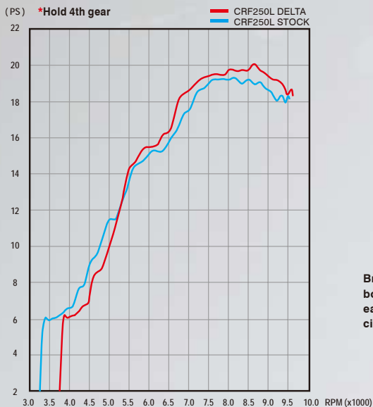
Provides more power and torque than stock pipes Dyno graph for CRF250L as shown above.
