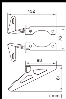
Tail light bracket Part number D45-18-130
